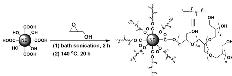
Scheme 1. Synthesis of ND functionalized with hyperbranched polyglycerol through the ring-opening polymerization of glycidol.
