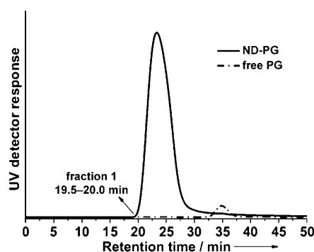
Figure 3. Chromatograms for the elution of ND-PG and free PG.
